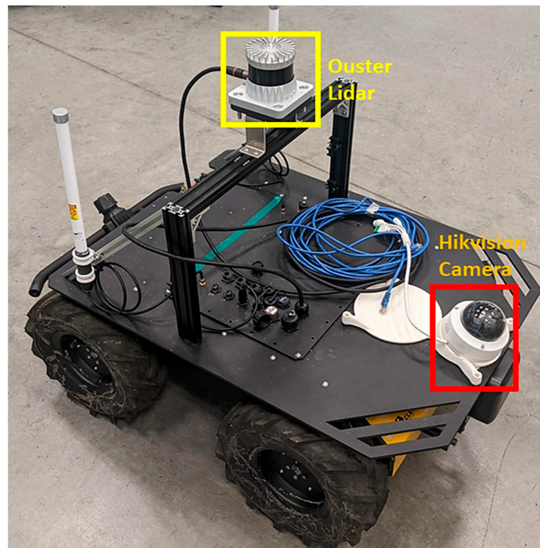
Figure 1. Husky robot setup with a Lidar sensor and Hikvision camera.
