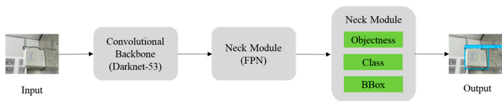
Figure 4. A flowchart of the charger detection method.
