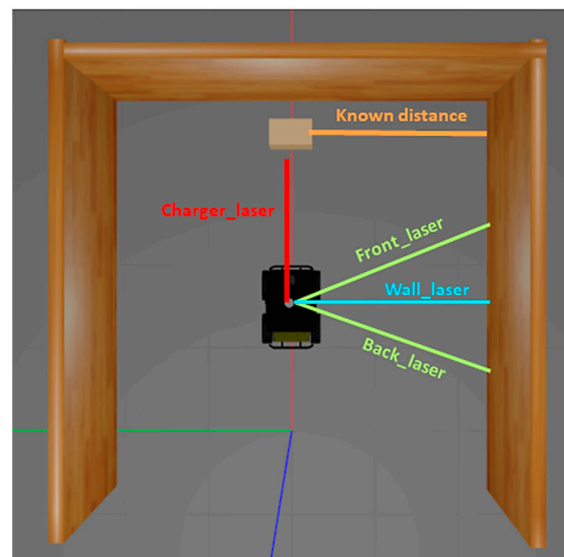
Figure 7. Lidar-based docking method visualization.
