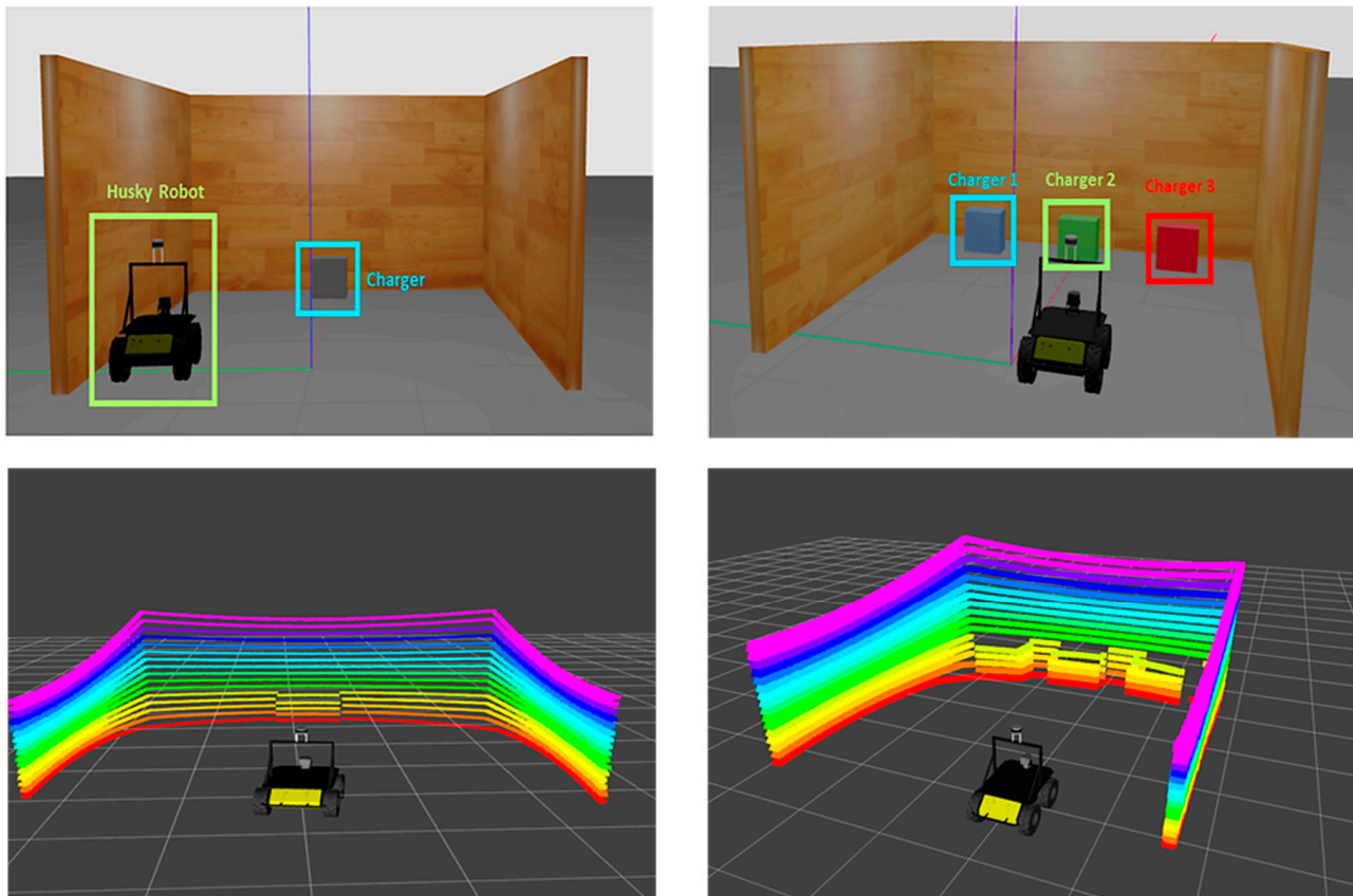
Figure 6. Docking station Gazebo virtual environment setup with one charger ( top left ) and three chargers ( top right ), and Rviz Lidar point cloud visualization for one charger ( bottom left ) and three chargers ( bottom right ).
